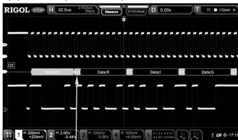
ACK = 1
