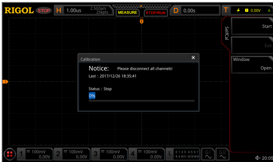
Figure 20-2 Self-calibration Interface
